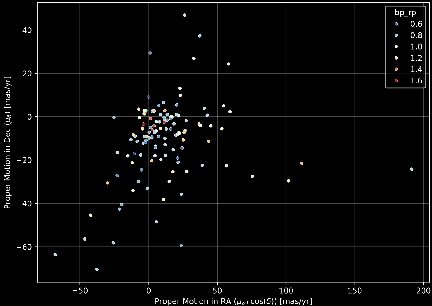
GALAH DR4 Field: [6680] Proper Motion Diagram (n= 120)
