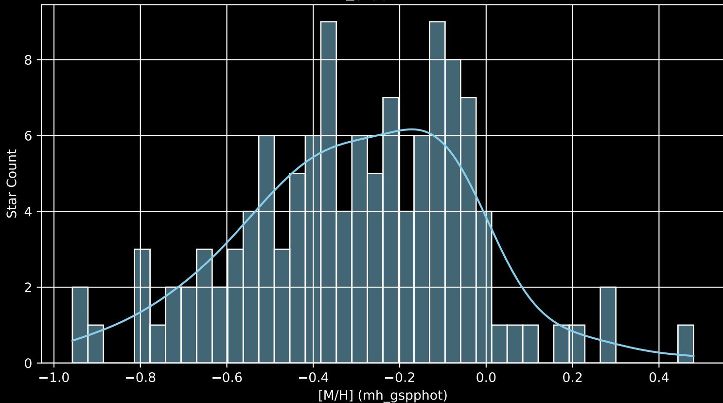
GALAH DR4 Field: [6680] [M/H] (mh_gspphot) (n= 120)
