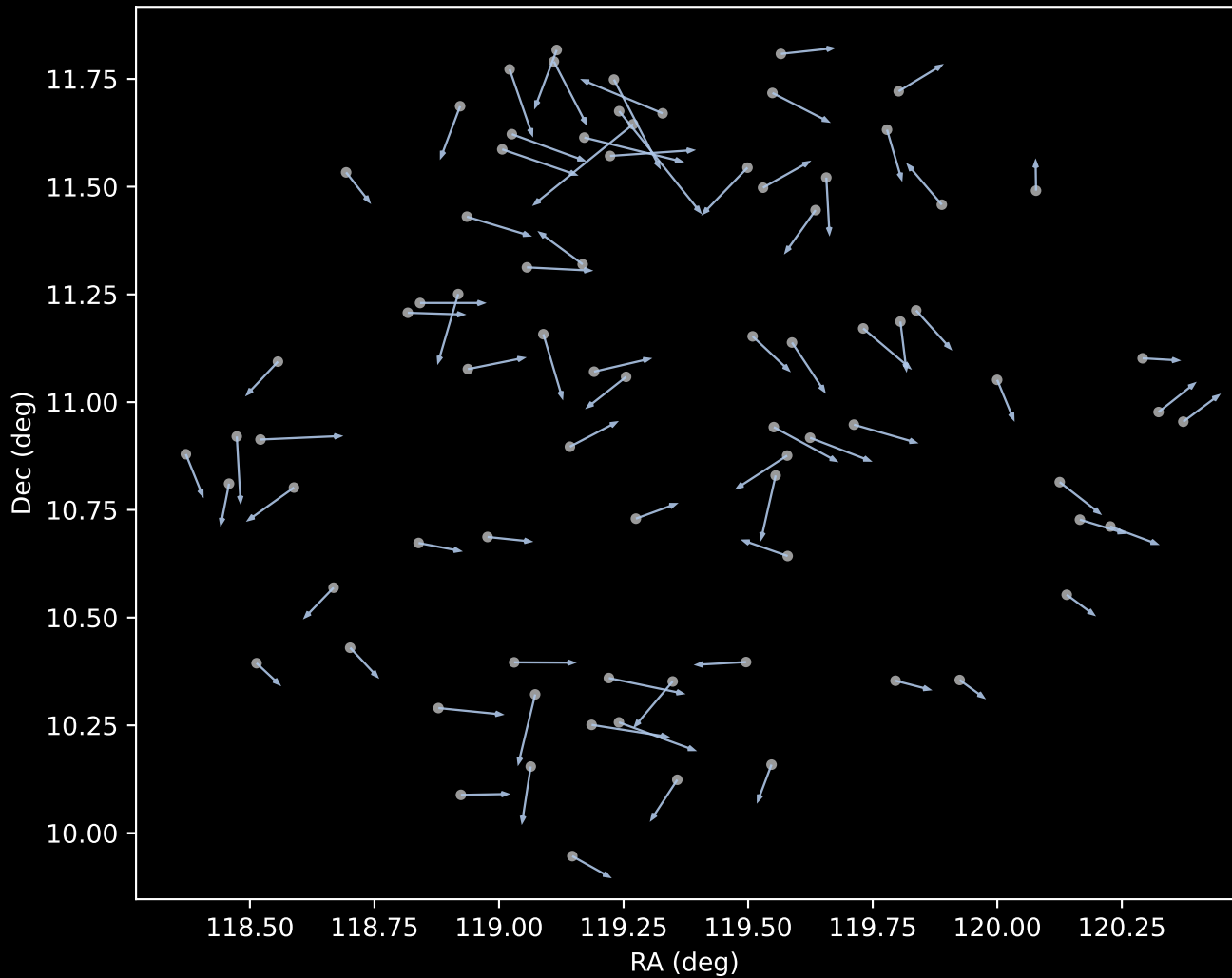
GALAH DR4 Cluster 1 Proper Motion Vectors (n=80)
