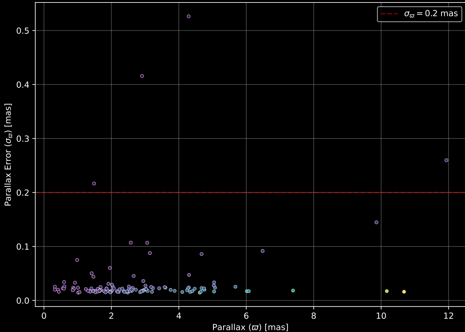
GALAH DR4 Field: [6680] Parallax Quality (n= 120)
