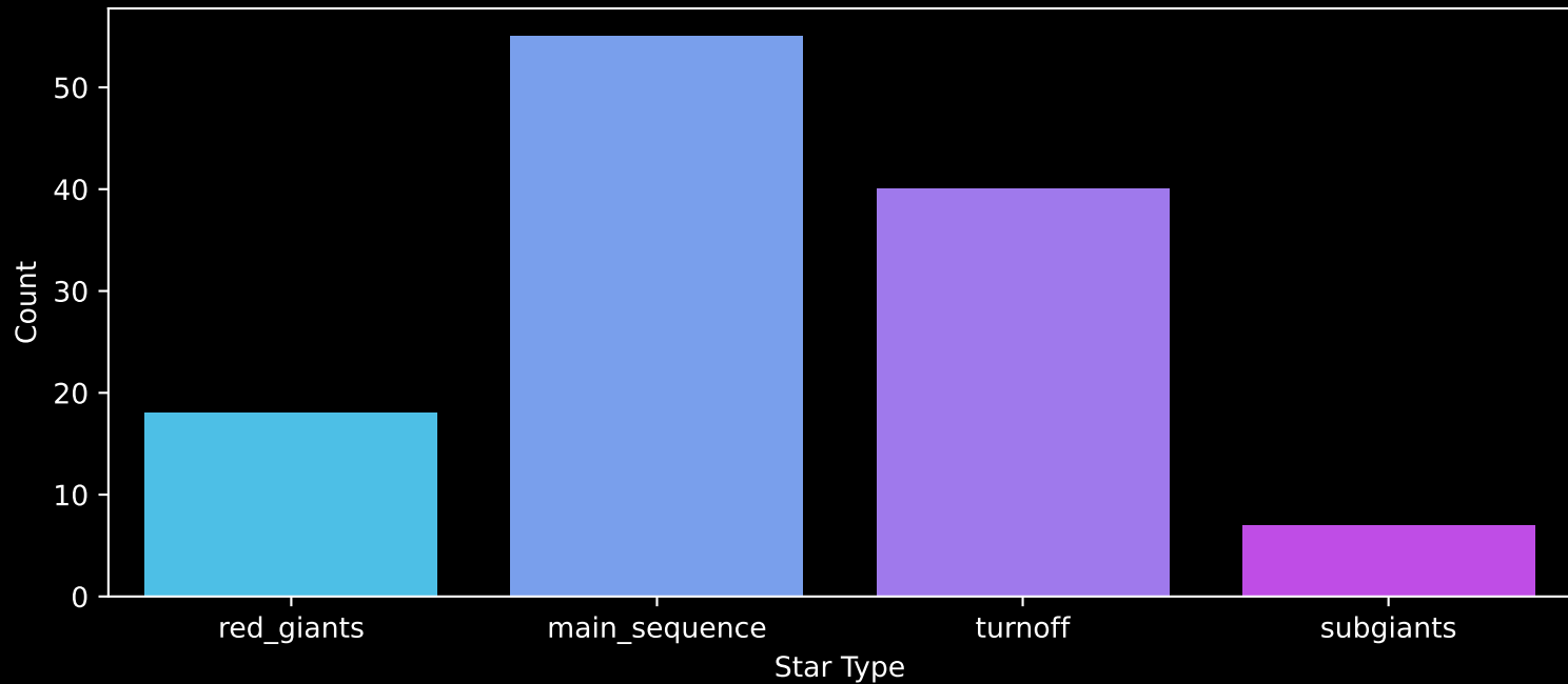
GALAH DR4 Field: [6680] Count plot of Star Type
