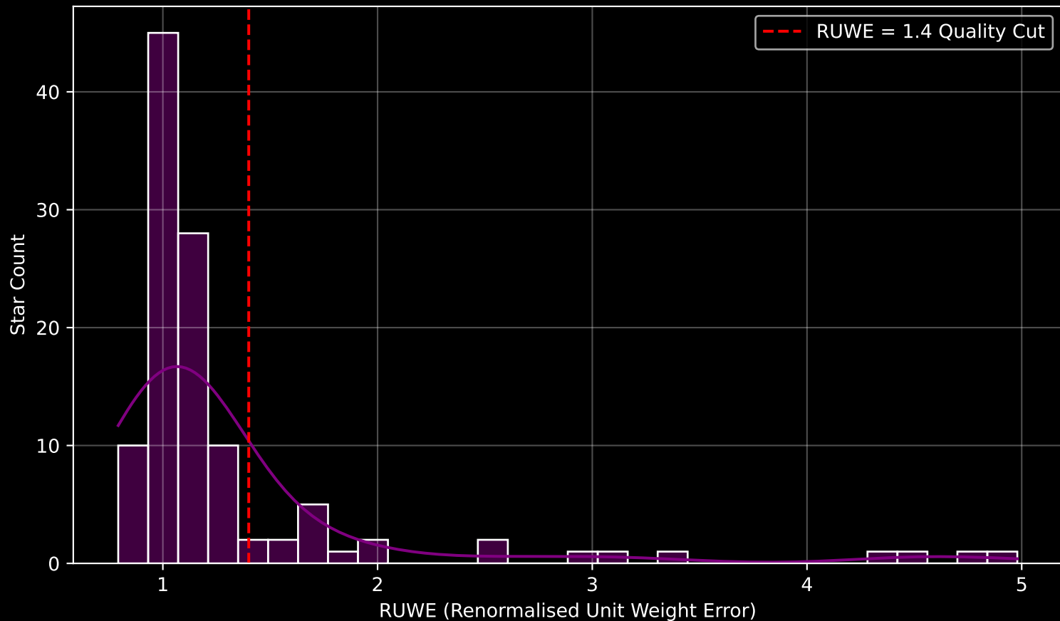
GALAH DR4 Field [6680] RUWE Distribution (n= 114)
